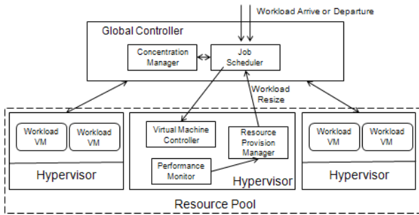
Figure 3. EnaCloud Architecture
